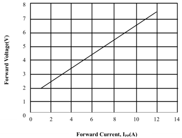
Forward Voltage vs. Forward Peak Pulse Current ( t_{period}=100ns, t_r=1ns )
