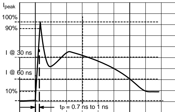
IEC61000-4-2 Waveform
