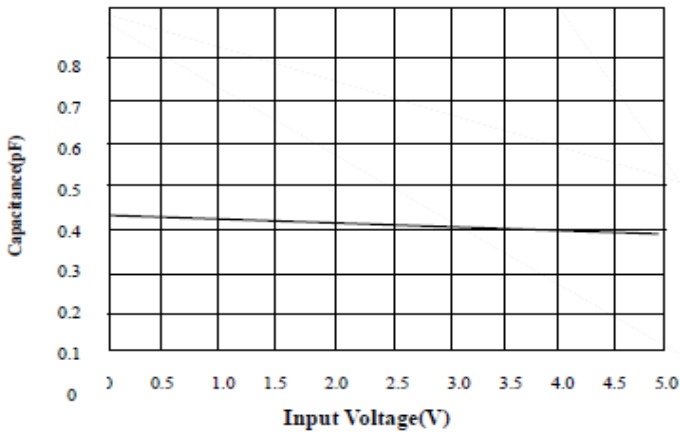
Typical Variation of CIN vs. VIN
