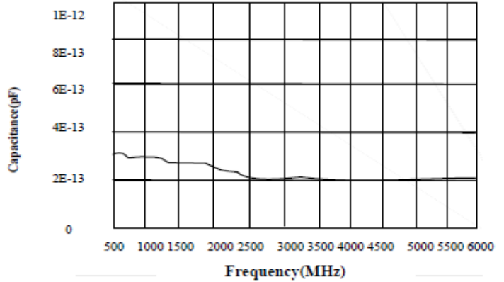
Capacitance vs. Frequency (IO to GND)
